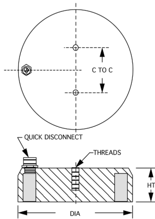
CE Series MODELS HAVE TOP WIRE OUTLET
