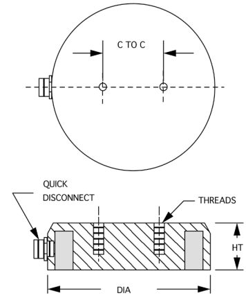
DC Series MODELS HAVE SIDE WIRE OUTLET
