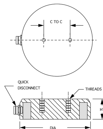
DC Series MODELS HAVE SIDE WIRE OUTLET
